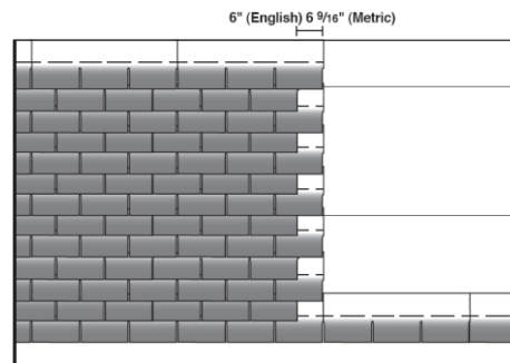
Racking Method
