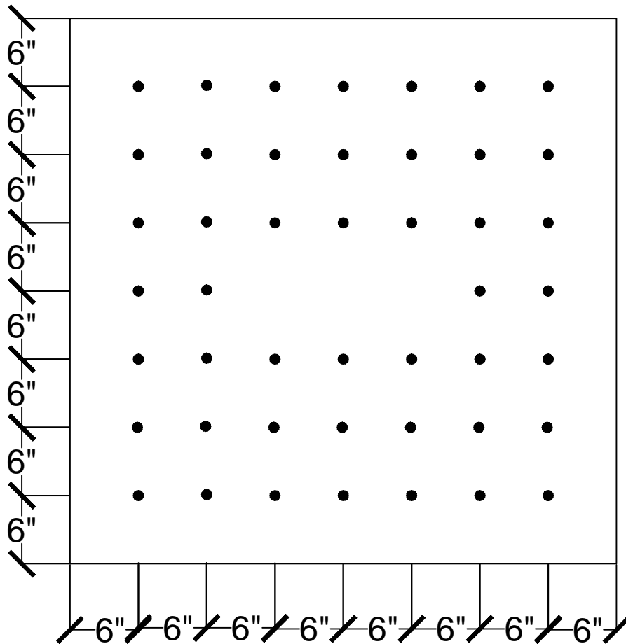
46 FASTENERS PER 4' x 4' BOARD
