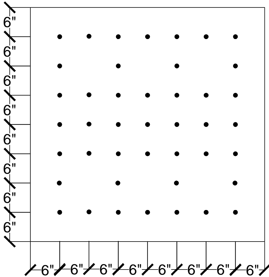
43 FASTENERS PER 4' x 4' BOARD
