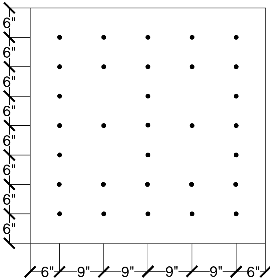
31 FASTENERS PER 4' x 4' BOARD
