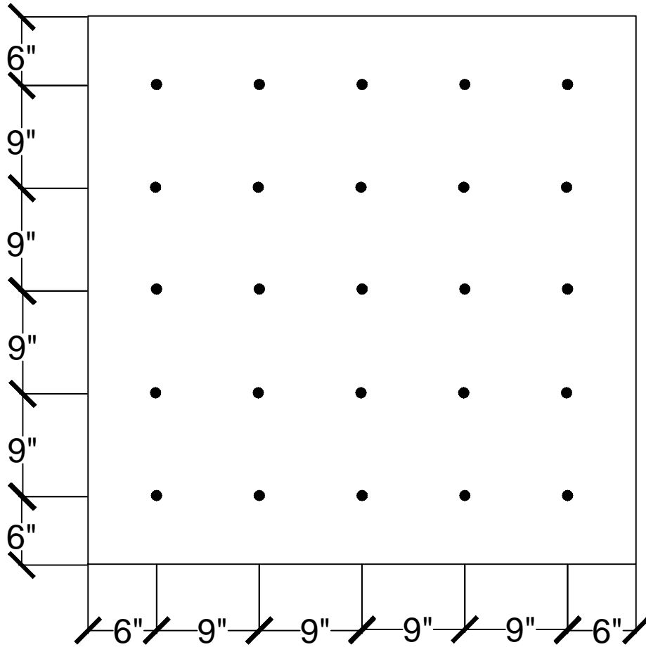
25 FASTENERS PER 4' x 4' BOARD
