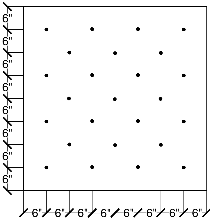
24 FASTENERS PER 4' x 4' BOARD
