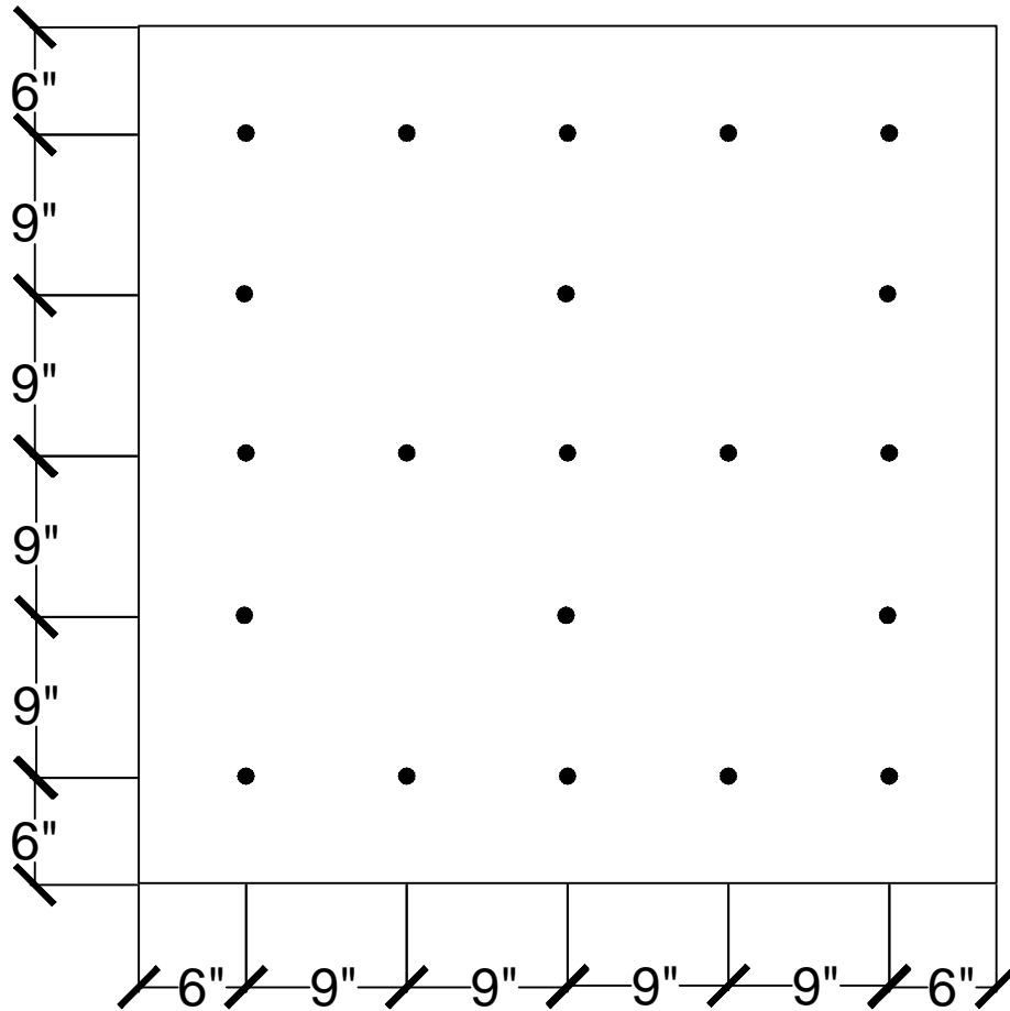
21 FASTENERS PER 4' x 4' BOARD
