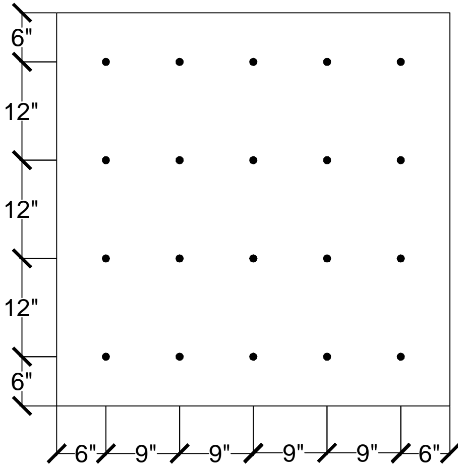
20 FASTENERS PER 4' x 4' BOARD
