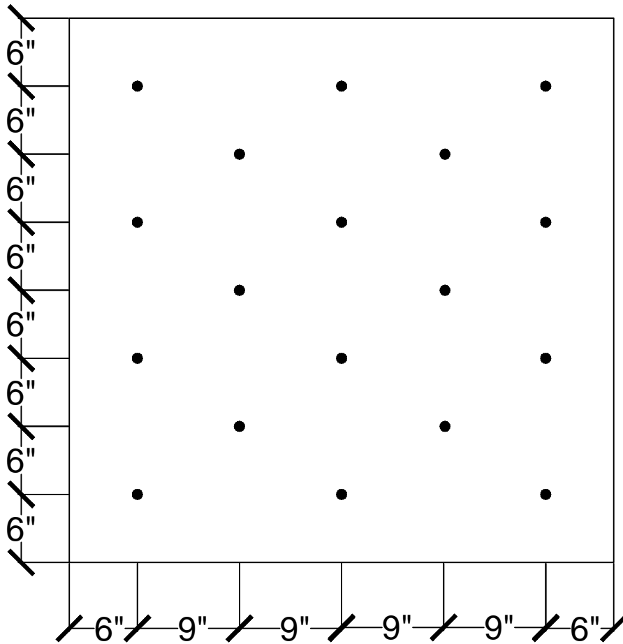
18 FASTENERS PER 4' x 4' BOARD
