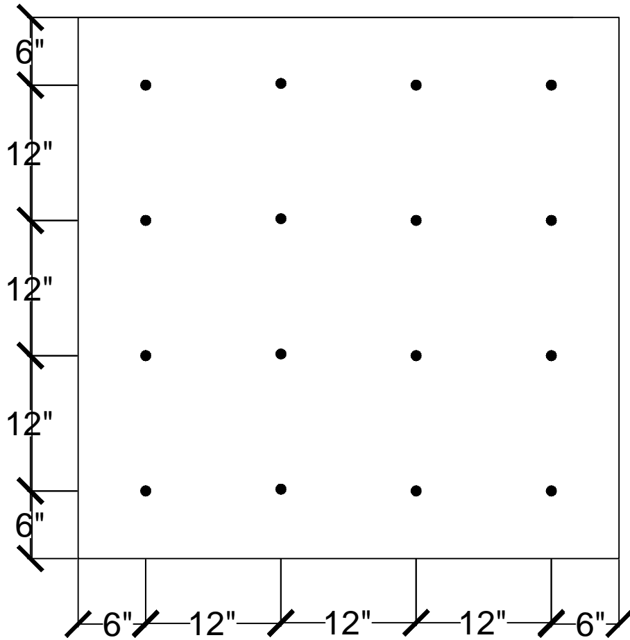
16 FASTENERS PER 4' x 4' BOARD
