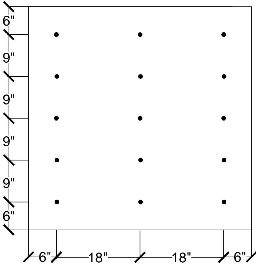
15 FASTENERS PER 4' x 4' BOARD
