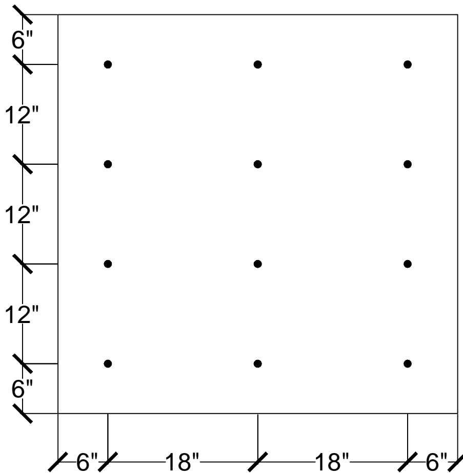
12 FASTENERS PER 4' x 4' BOARD
