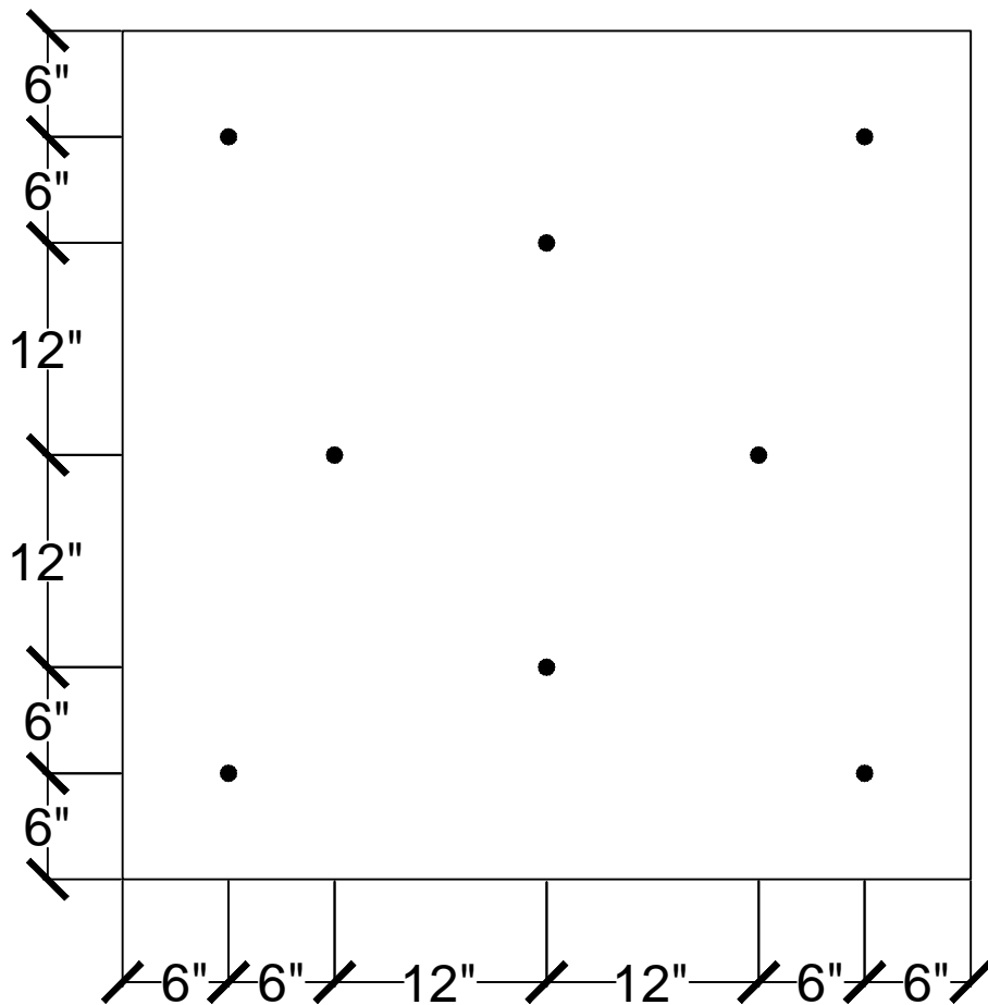
8 FASTENERS PER 4' x 4' BOARD
