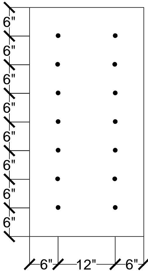
14 FASTENERS PER 2' x 4' BOARD
