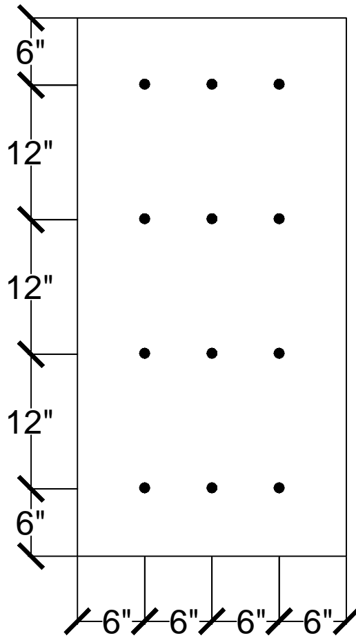
12 FASTENERS PER 2' x 4' BOARD
