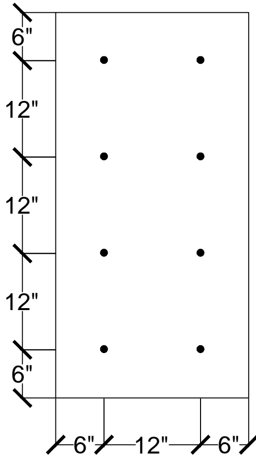
8 FASTENERS PER 2' x 4' BOARD
