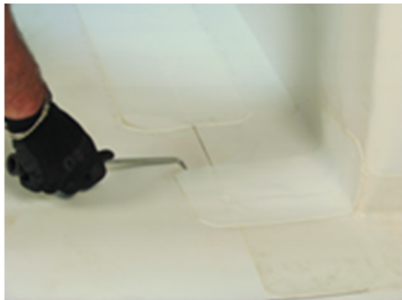
Fig. 1: Seaming Probing
