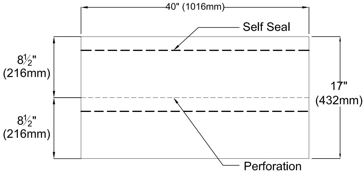
Full WeatherBlocker™ Starter Strip Shingle used at eaves with shingles with exposures of at least 6".
