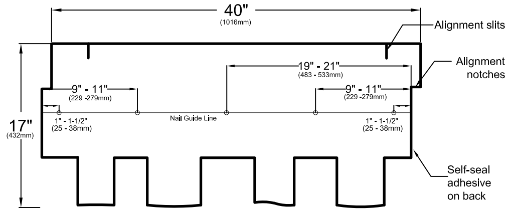
STANDARD NAILING PATTERN - five nails per shingle
