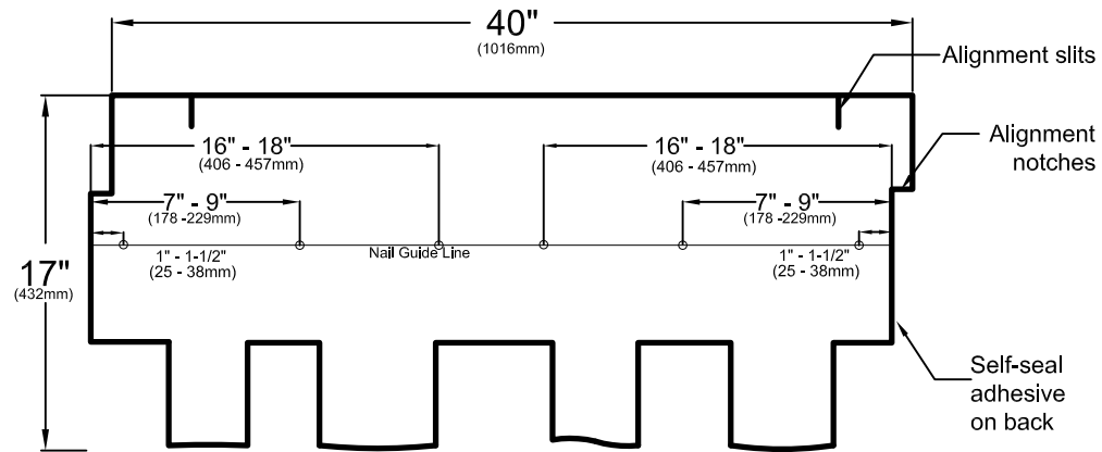
ENHANCED NAILING PATTERN - six nails per shingle*
