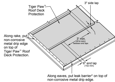
Figure 1 – Standard Application For 4:12 Slope Or More
