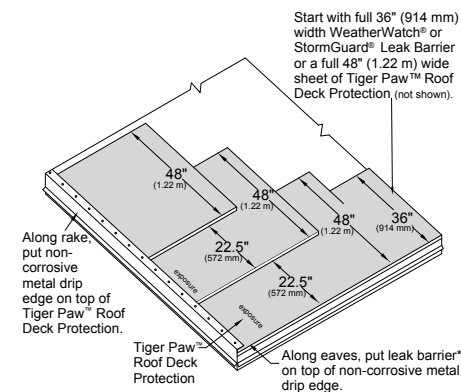
Figure 2 – Standard Application For Low Slopes (2:12 Slope Up To But Not Including 4:12)
