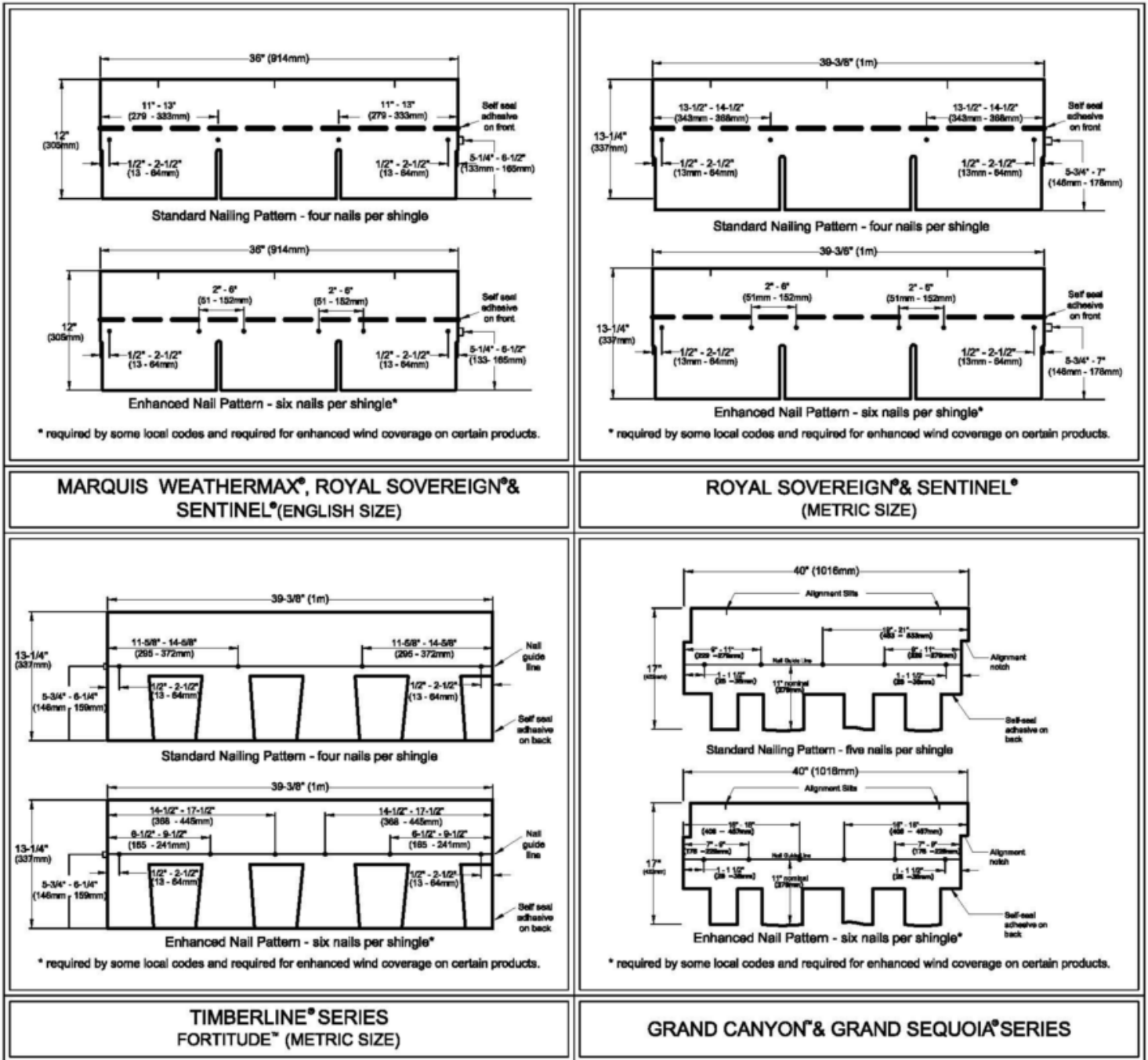
FIGURE 1—GAF SHINGLES
