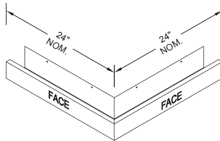
OUTSIDE MITER
