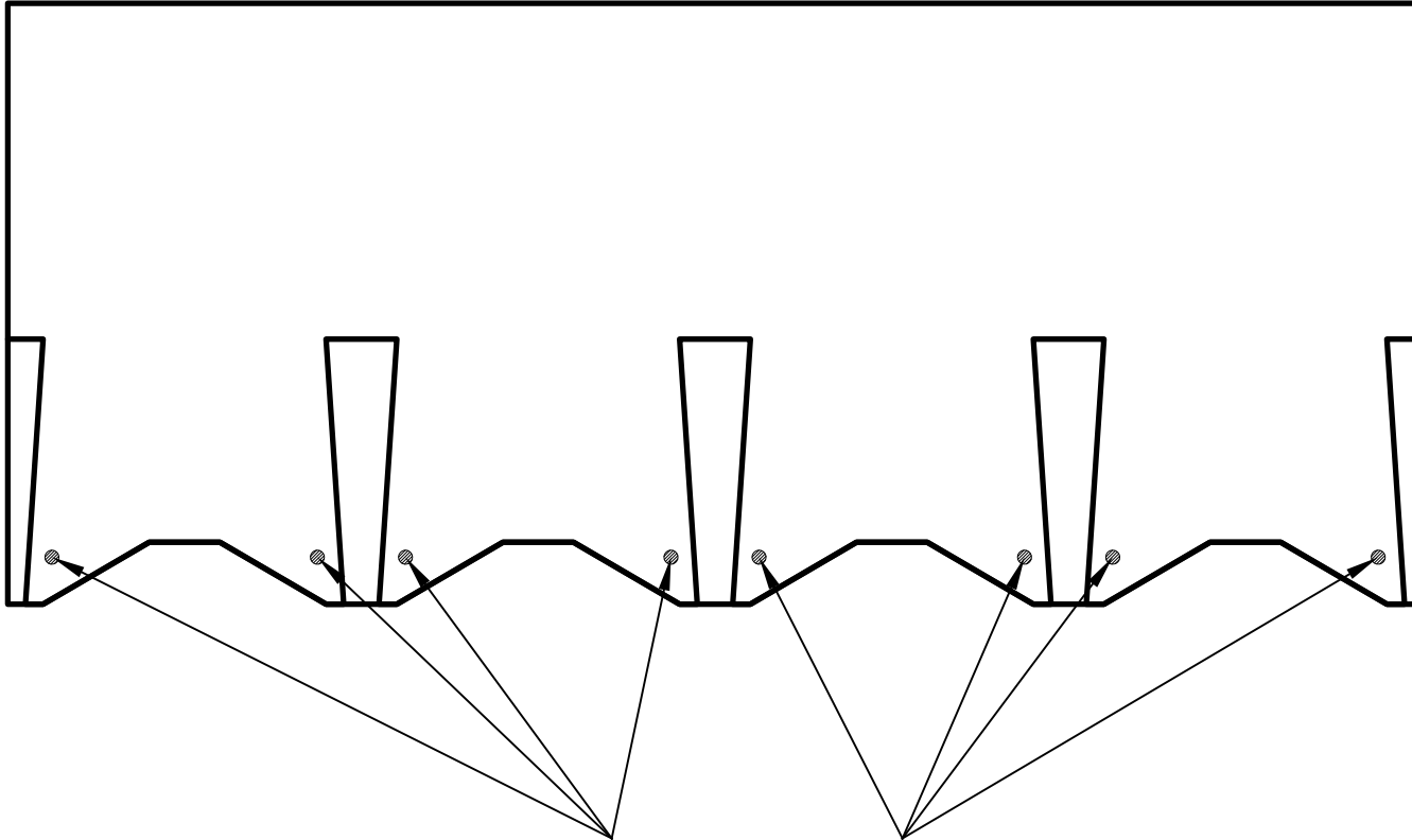
Cement locations (8 quarter-sized dabs of cement on back of shingle)
