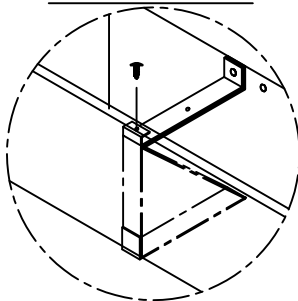
FASTENER DETAIL
