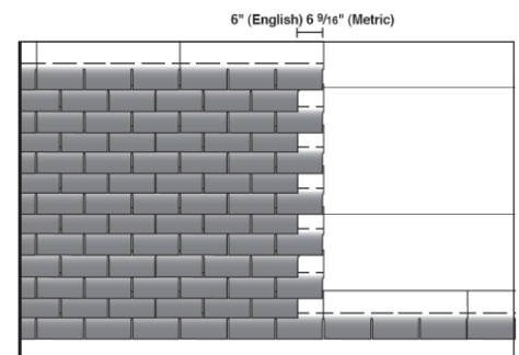
Racking Method
