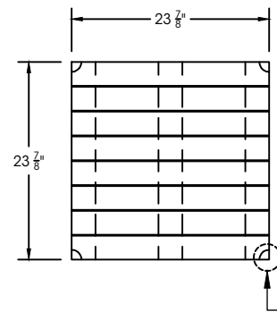
Plan GRT wood deck tile
