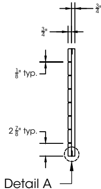
Side Elevation GRT wood deck tile
