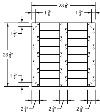
Bottom Elevation GRT wood deck tile
