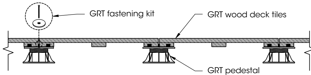
GRT Wood Deck Tile Application 2 GRT wood deck tiles on pedestals
