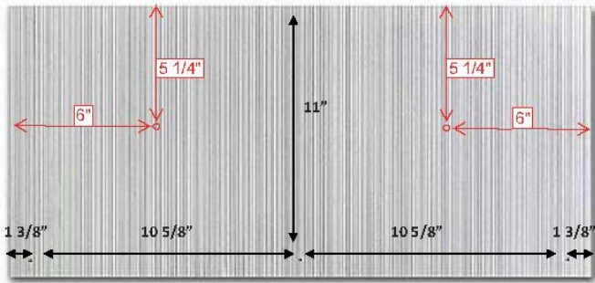
Figure 2: Profile 12, 5-nails/shingle
