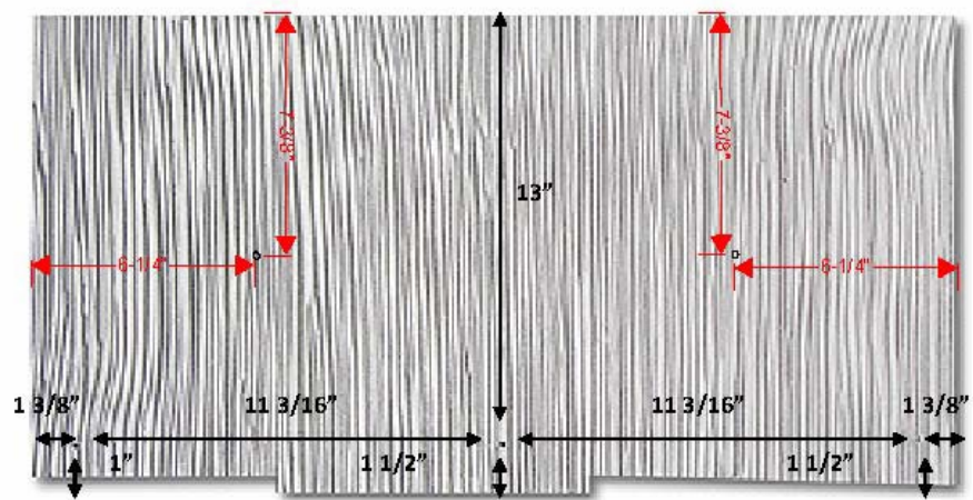
Figure 6: Emphasis™, 5-nails/shingle
