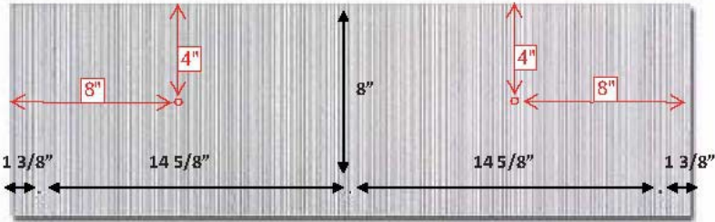
Figure 1: Profile 9, 5-nails/shingle
