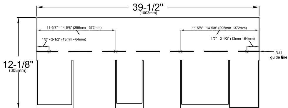
STANDARD NAILING PATTERN - four nails per shingle
