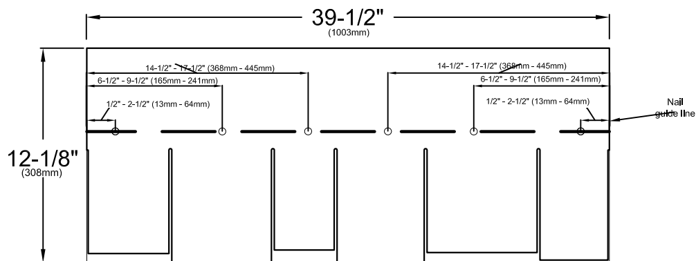
ENHANCED NAILING PATTERN - six nails per shingle*
