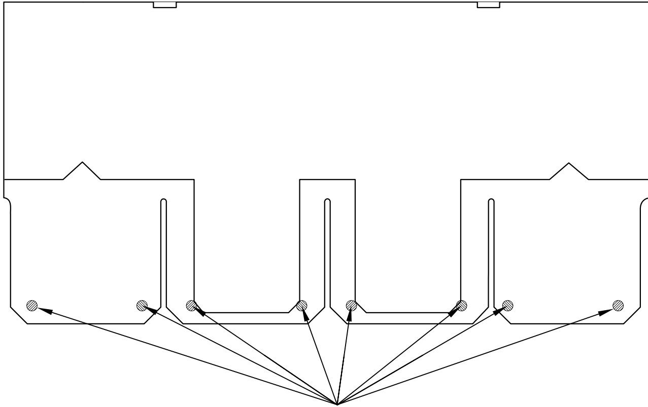
Cement locations (8 quarter-sized dabs of cement on back of shingle)
