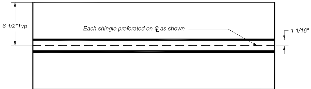
TOP VIEW
