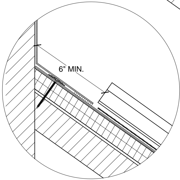
ALTERNATE - TERMINATE 6" MIN. FROM HEAD WALL
