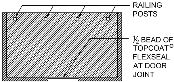
PLAN VIEW OF BALCONY
