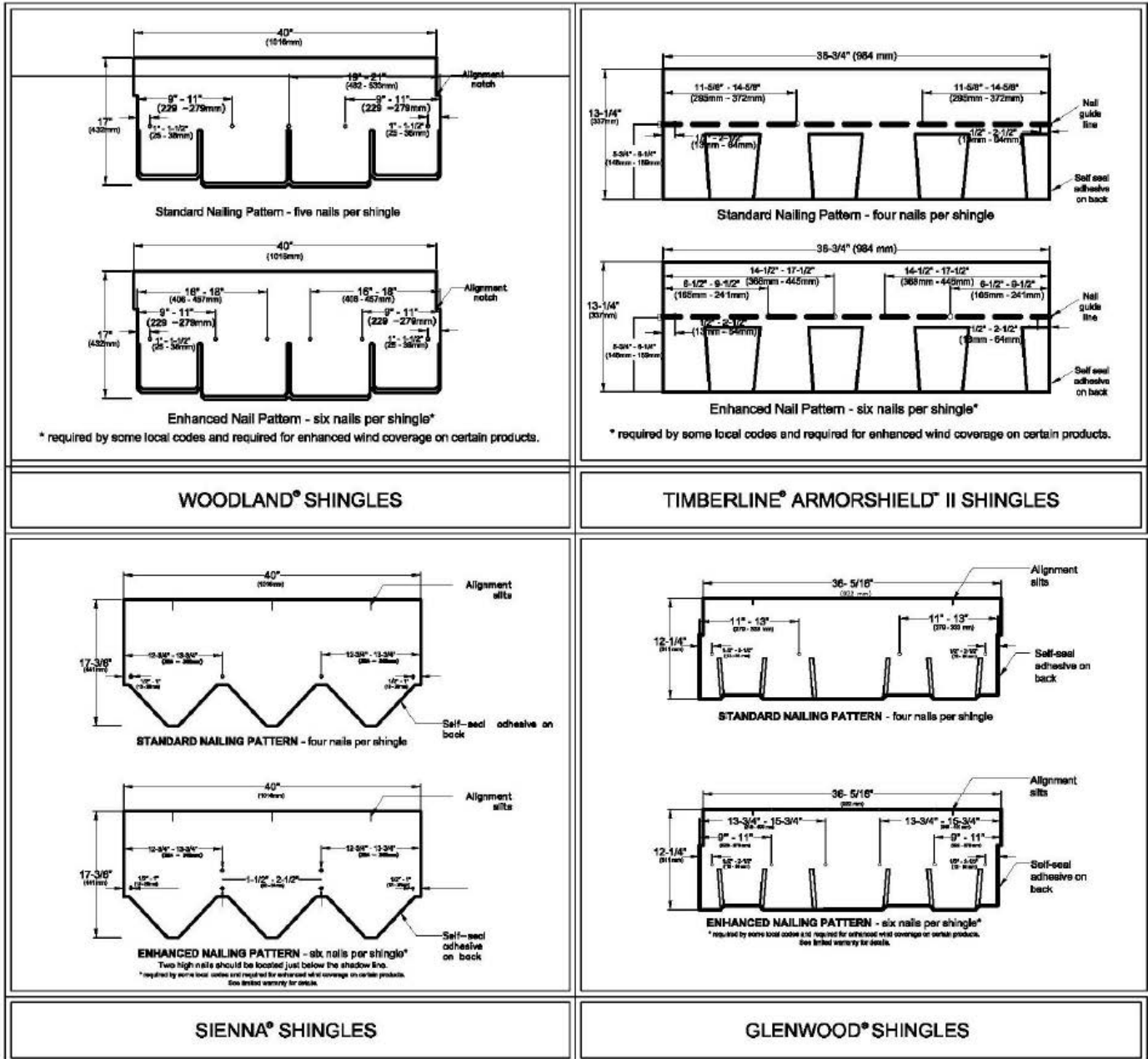
FIGURE 1—GAF SHINGLES (Continued)
