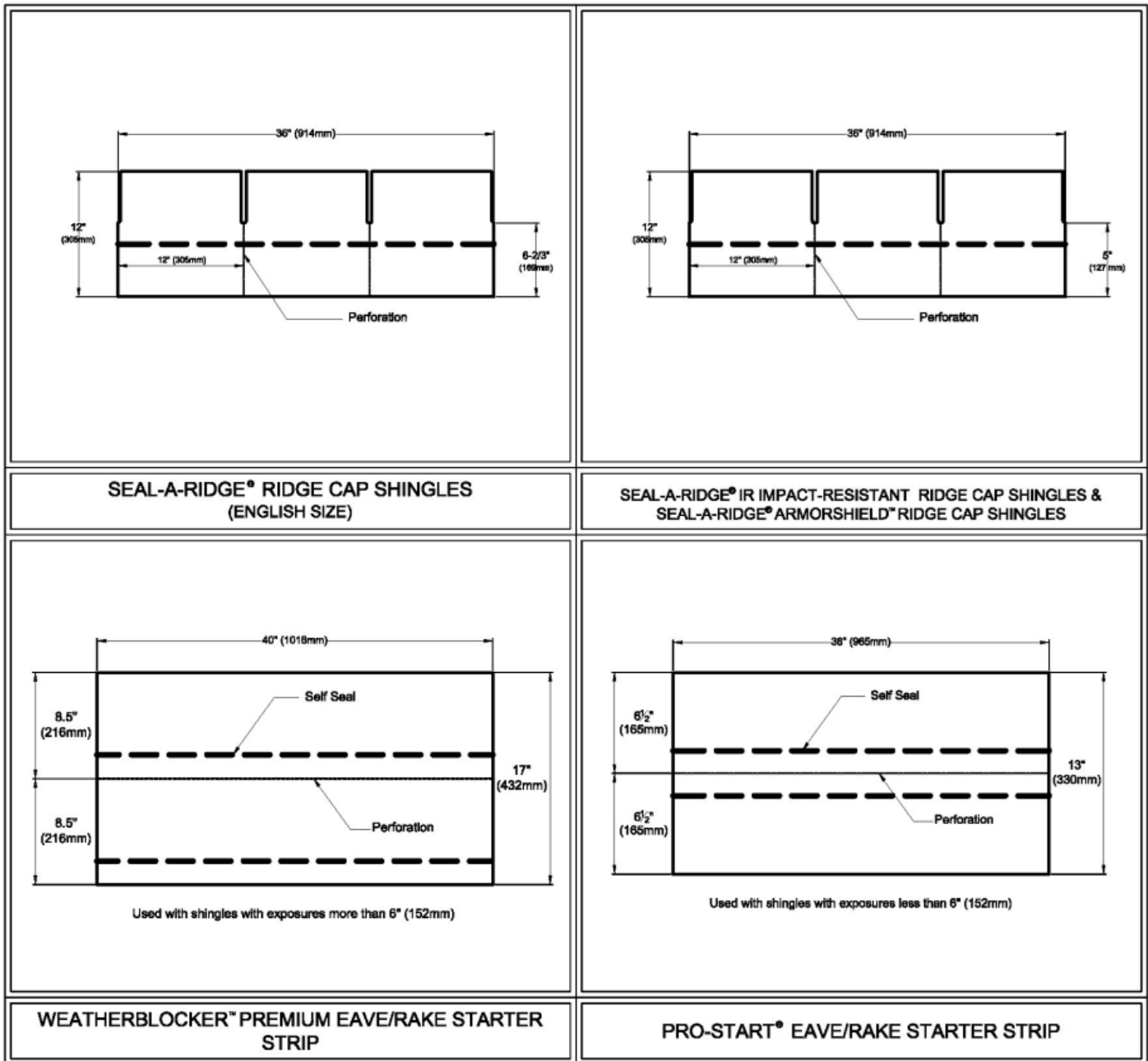
FIGURE 3—RIDGE AND STARTER SHINGLES
