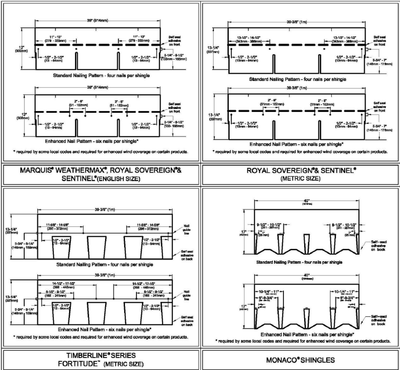
FIGURE 1—GAF SHINGLES
