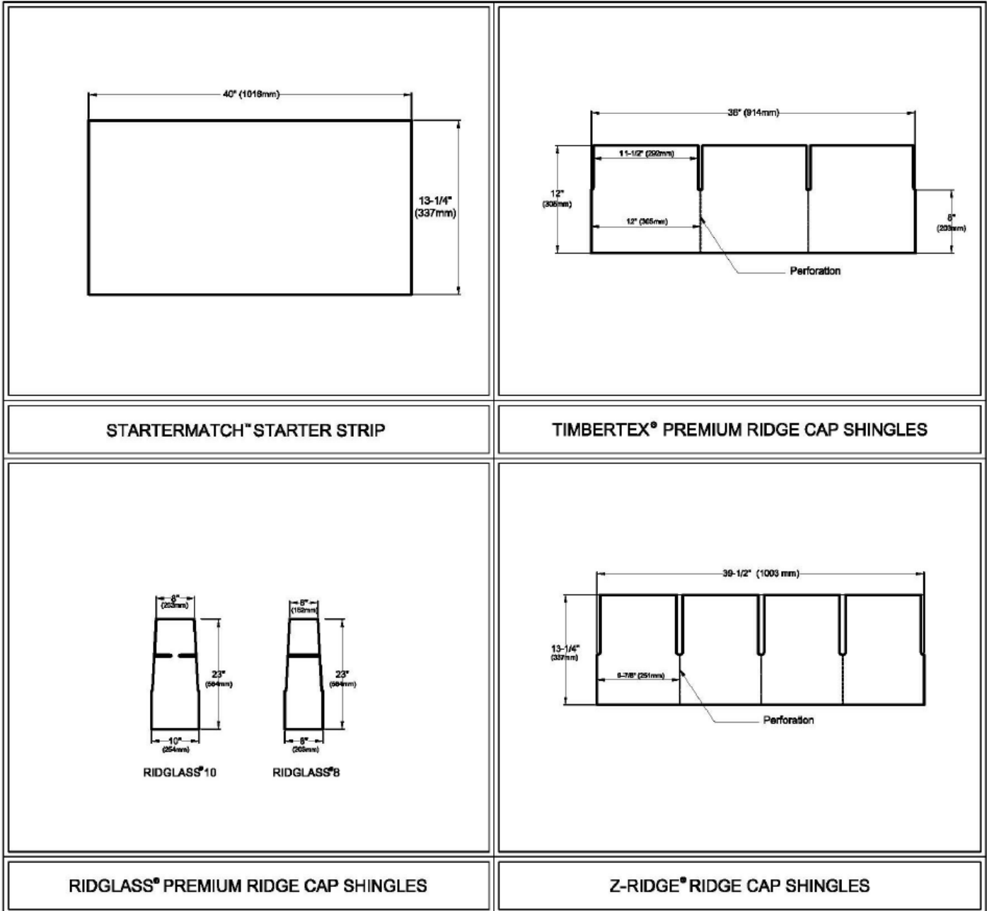
FIGURE 2—STARTER AND RIDGE SHINGLES
