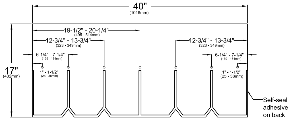
ENHANCED NAILING PATTERN - seven nails per shingle*
