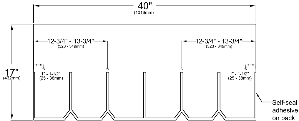
STANDARD NAILING PATTERN - four nails per shingle
