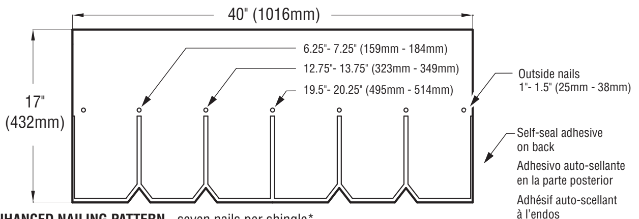
ENHANCED NAILING PATTERN - seven nails per shingle*
