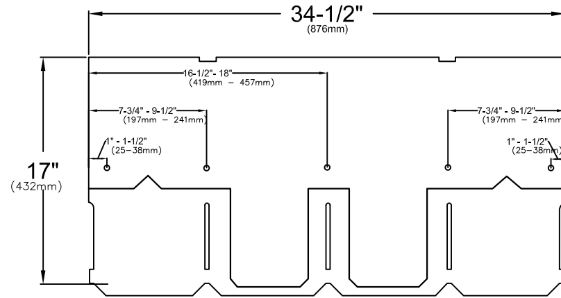
STANDARD NAILING PATTERN - five nails per shingle
