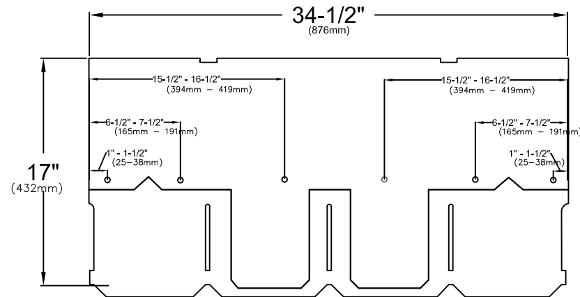
ENHANCED NAILING PATTERN - six nails per shingle*
