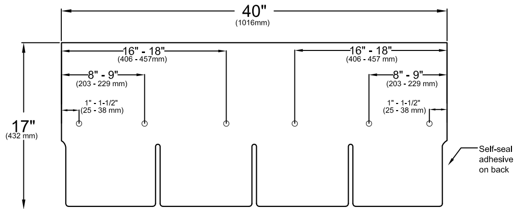
ENHANCED NAILING PATTERN - six nails per shingle*
