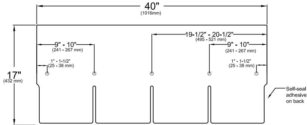
STANDARD NAILING PATTERN - five nails per shingle
