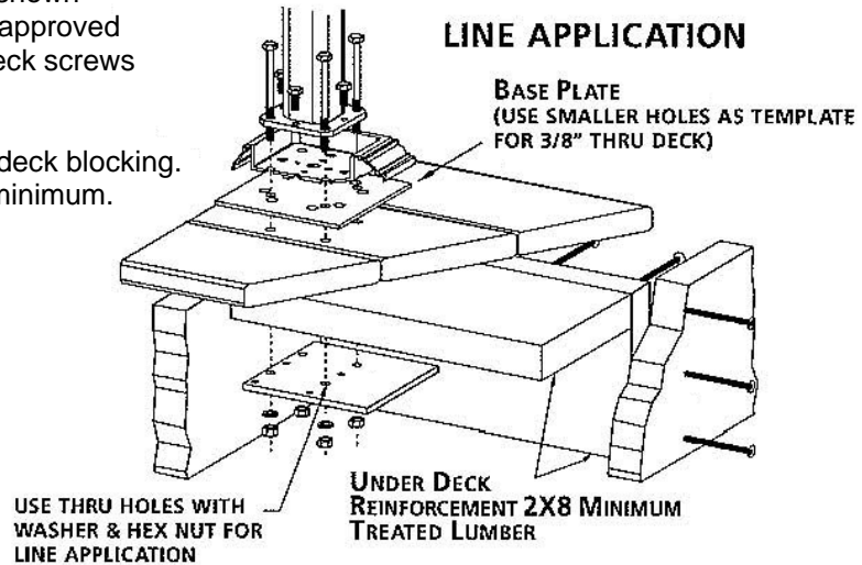
Figure 6 – UltiMount™ Installation on a Wood Deck
