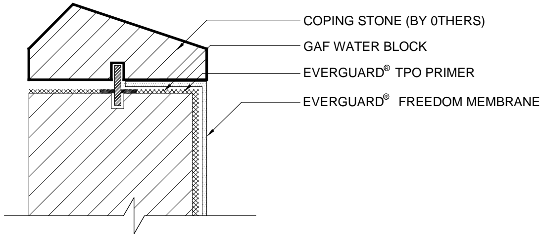
4. COPING STONE TERMINATION
