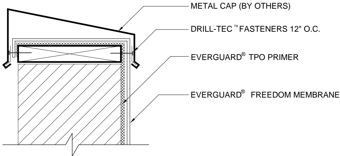
5. CAP FLASHING TERMINATION
