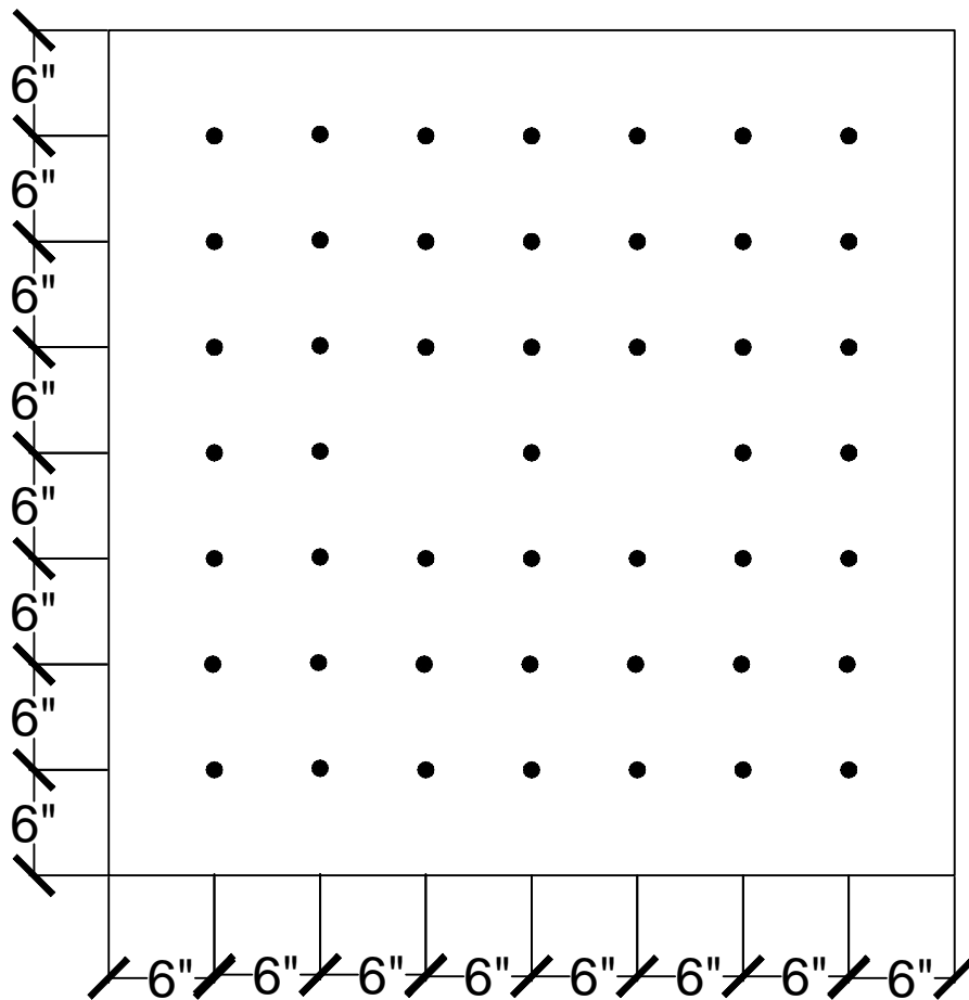
47 FASTENERS PER 4' x 4' BOARD
