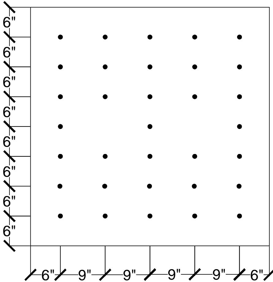
33 FASTENERS PER 4' x 4' BOARD
