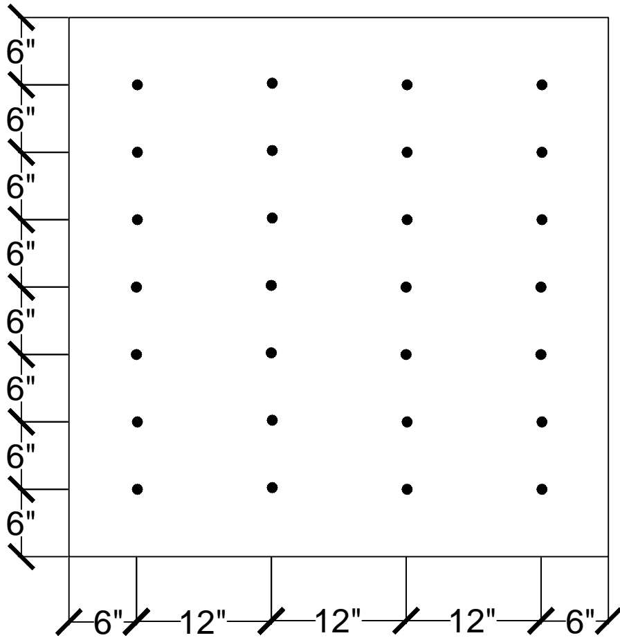
28 FASTENERS PER 4' x 4' BOARD
