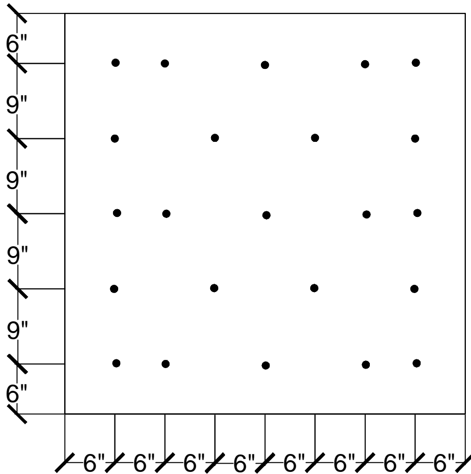
23 FASTENERS PER 4' x 4' BOARD
