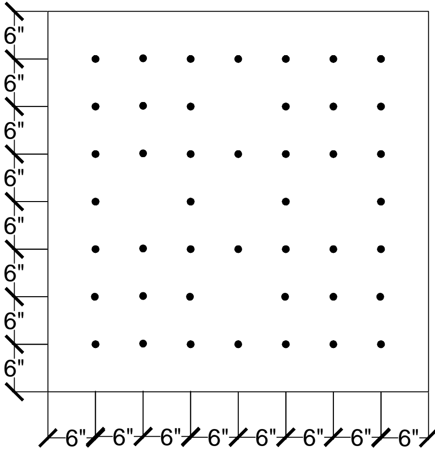
44 FASTENERS PER 4' x 4' BOARD
