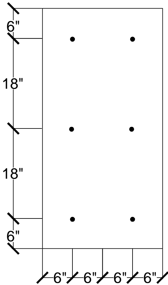
6 FASTENERS PER 2' x 4' BOARD
