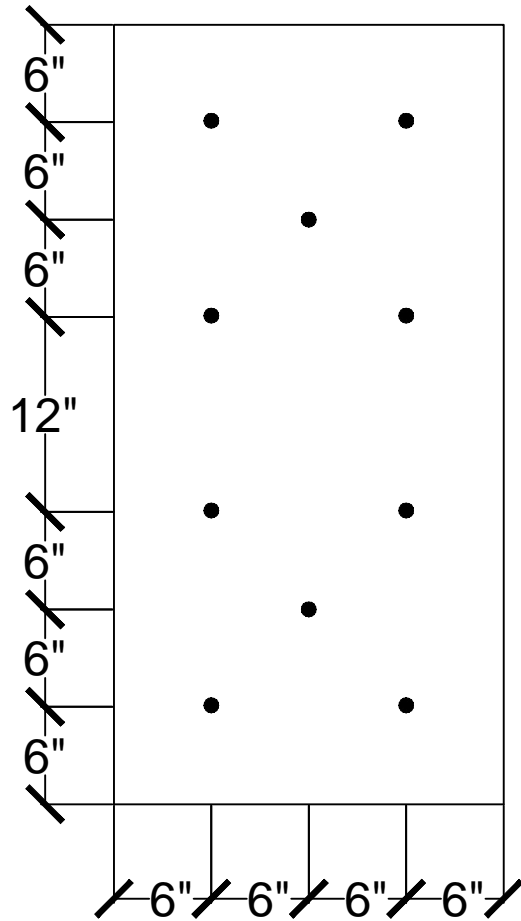
10 FASTENERS PER 2' x 4' BOARD
