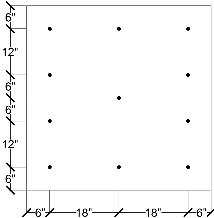
11 FASTENERS PER 4' x 4' BOARD
