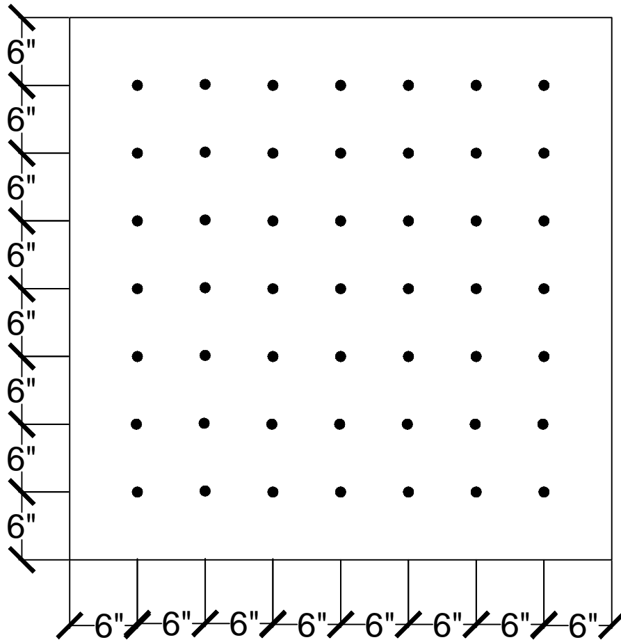
49 FASTENERS PER 4' x 4' BOARD
