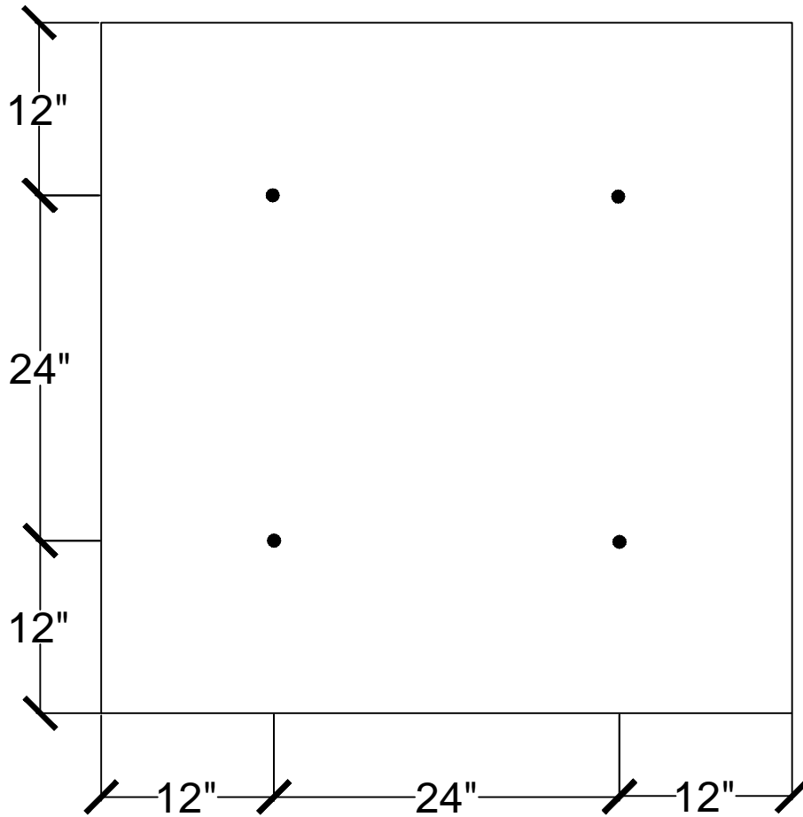
4 FASTENERS PER 4' x 4' BOARD
