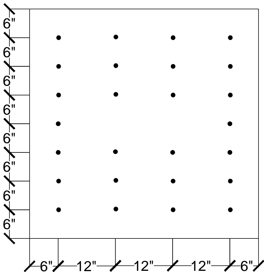
26 FASTENERS PER 4' x 4' BOARD
